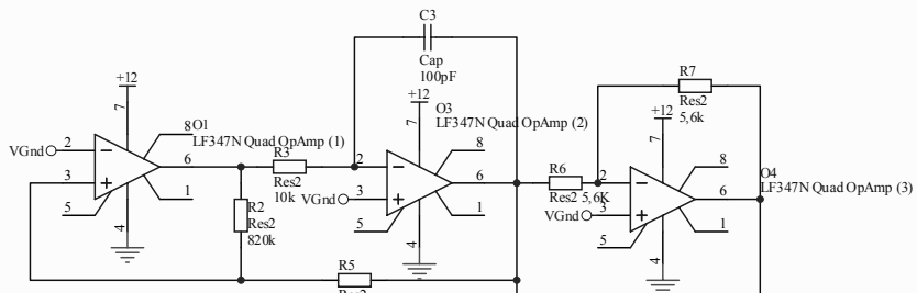
Triangle Wave Generator
