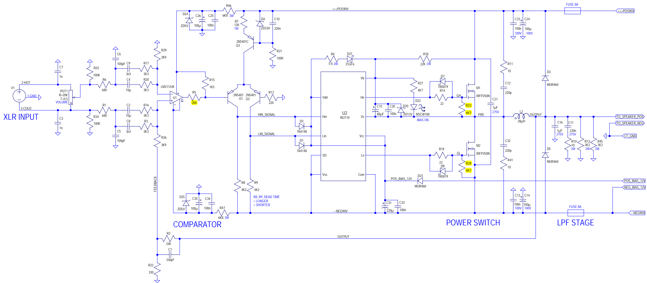
UcD-1K -- HB UcD IR2110 Class D BASIC Ver.1a Kartino Surodipo - Copyright Nov 2021 ATTENTION: NOT FOR SALE UNLESS PERMITTED! Contact: kartino.id@gmail.com Indonesian - Class D Next Generation Facebook Group
