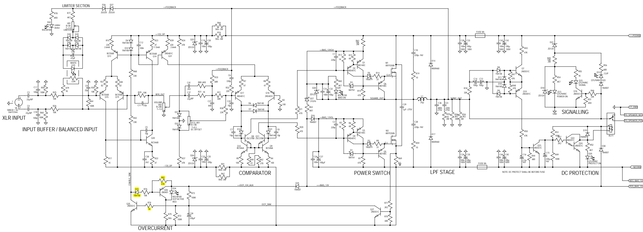
UcD-FD1K -- Fully Discrete HB UcD Class D Flagship Ver. 1a Kartino Surodipo - Copyright Sep 2021 ATTENTION: NOT FOR SALE UNLESS PERMITTED! Contact: kartino.id@gmail.com Indonesian - Class D Next Generation Facebook Group
