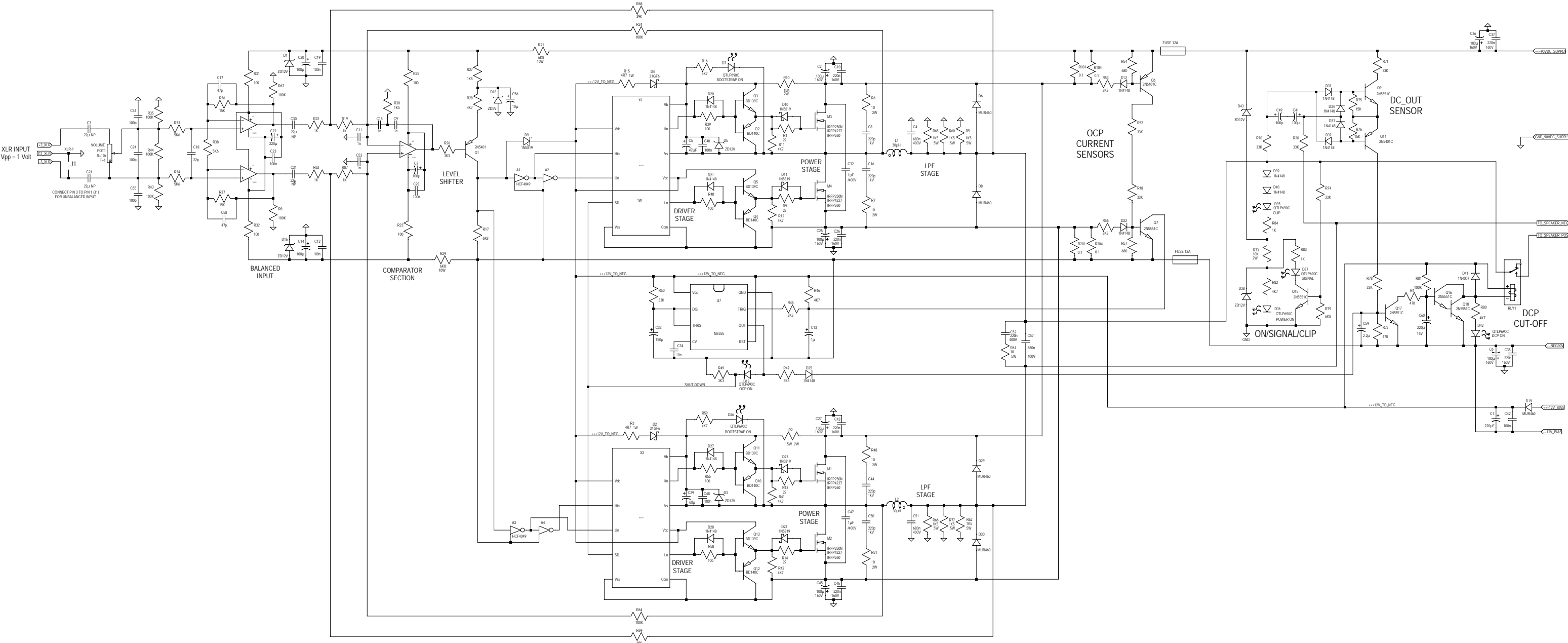
D2KFBNeo Full Bridge Class D Amplifier v.4 DOUBLE FEEDBACK FINALE Kartino Surodipo , August 2020
