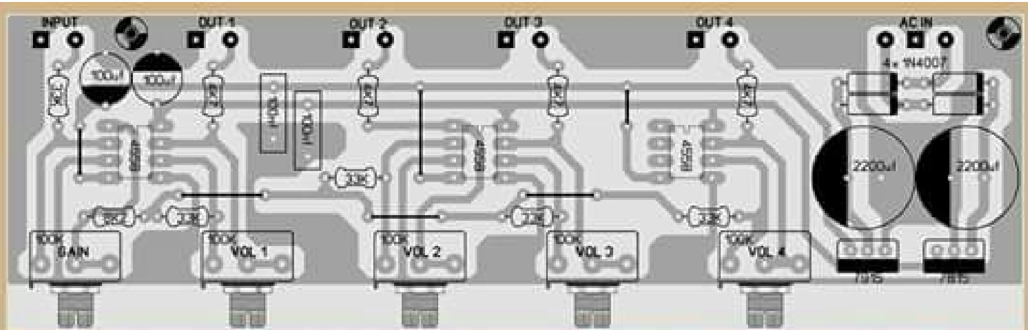
AUDIO DISTRIBUTOR ANWAR PCB 15 x 4 cm BY GEPENX
