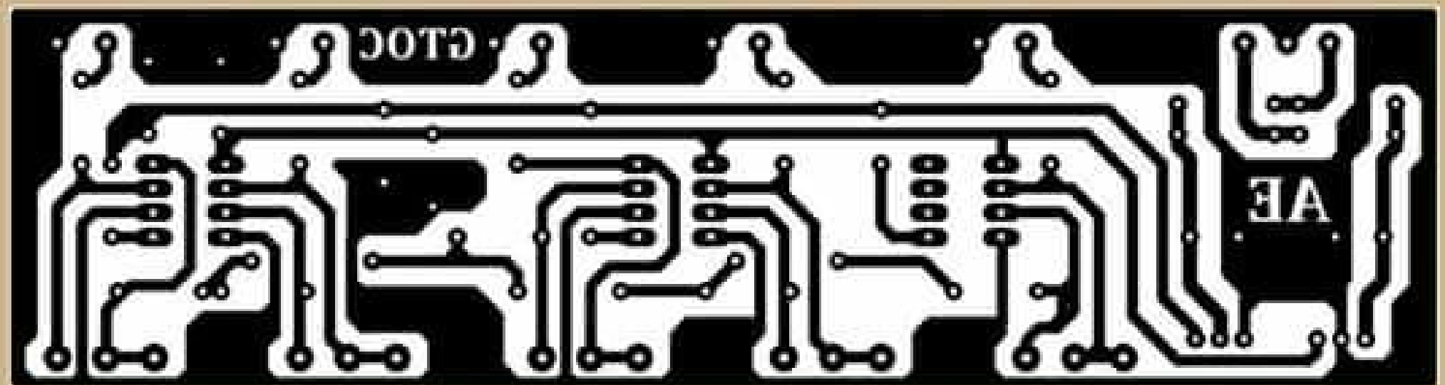
AUDIO DISTRIBUTOR ANWAR PCB 15 x 4 cm BY GEPENX
